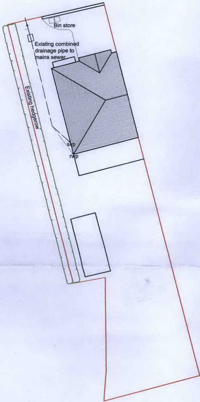
Existing block plan
